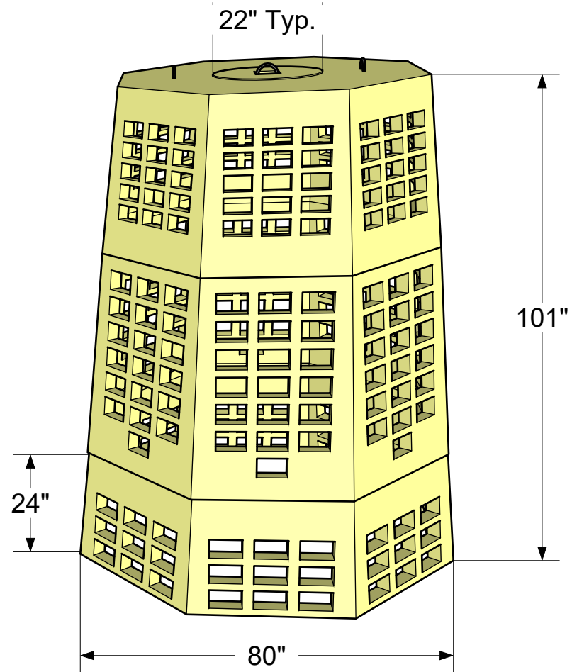
1500 Gallon Dry Well
