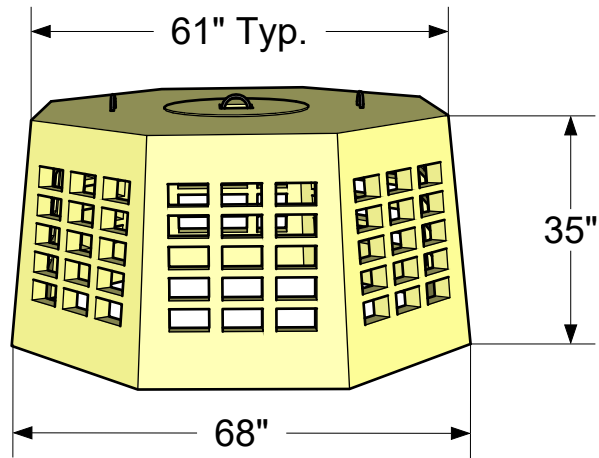
400 Gallon Dry Well
