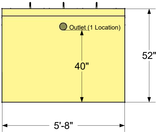
Tank Dimensions
